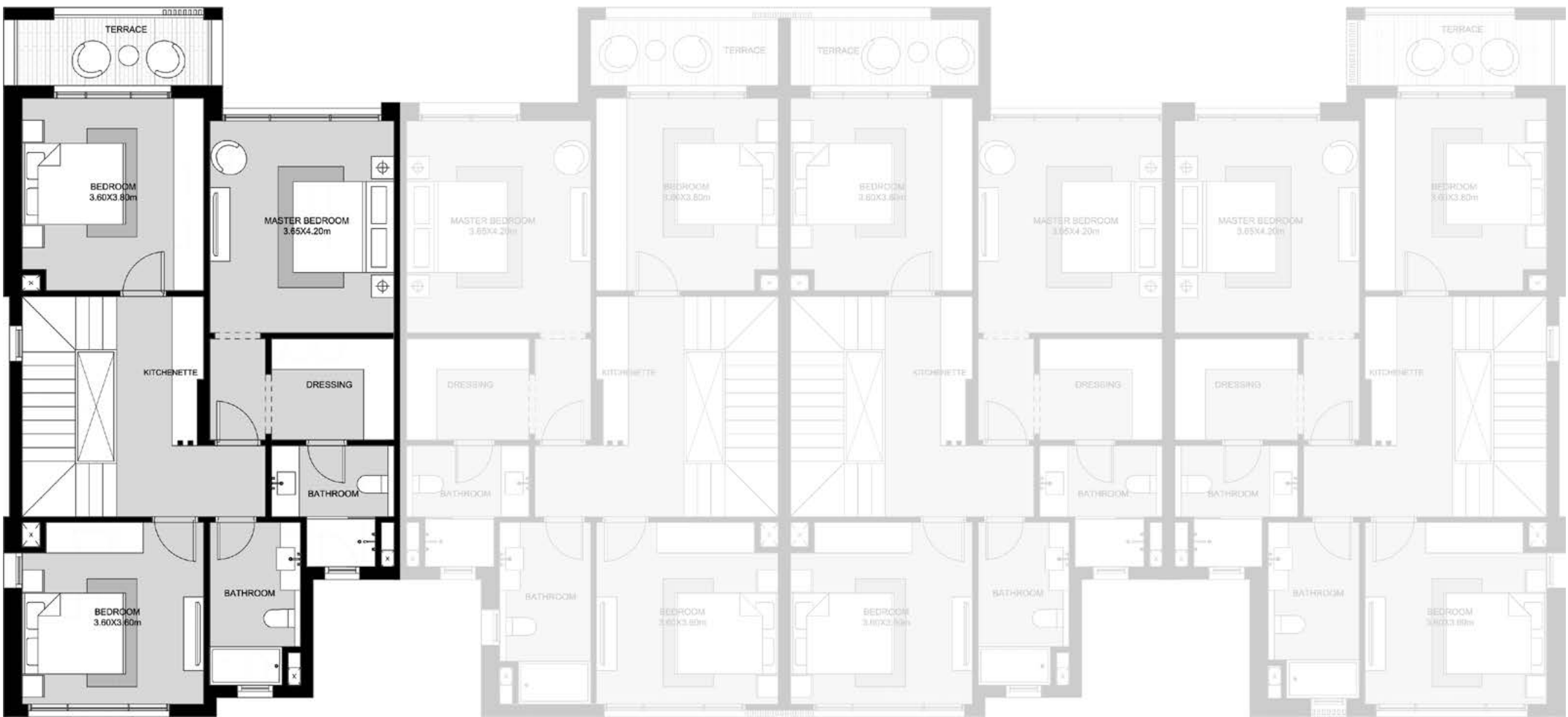
Ground Floor
