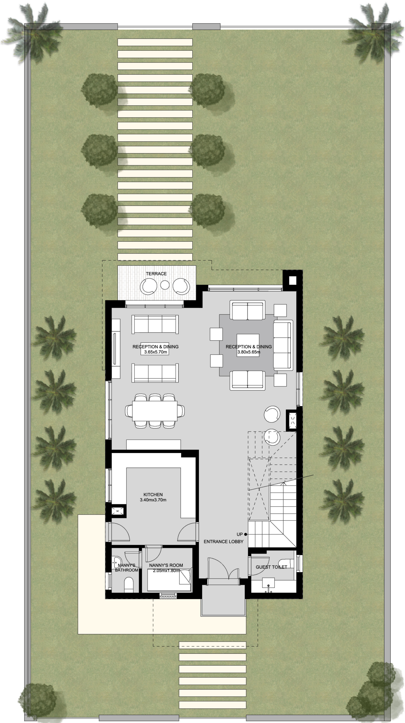
Ground Floor
