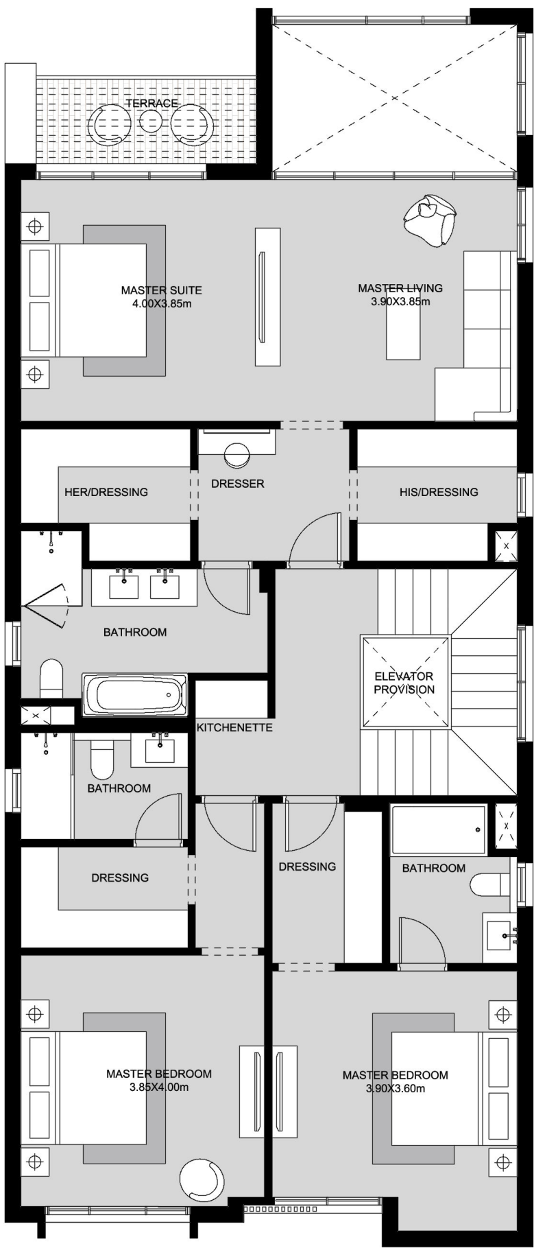
First Floor
