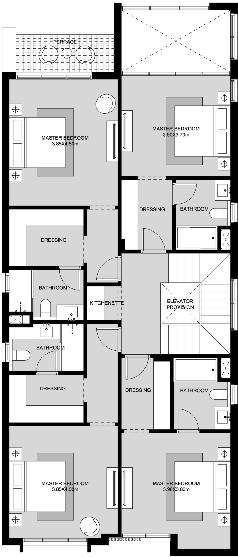
First Floor
