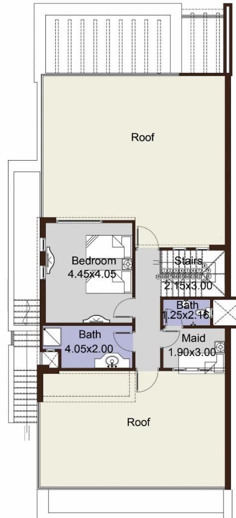
Roof Floor Plan
