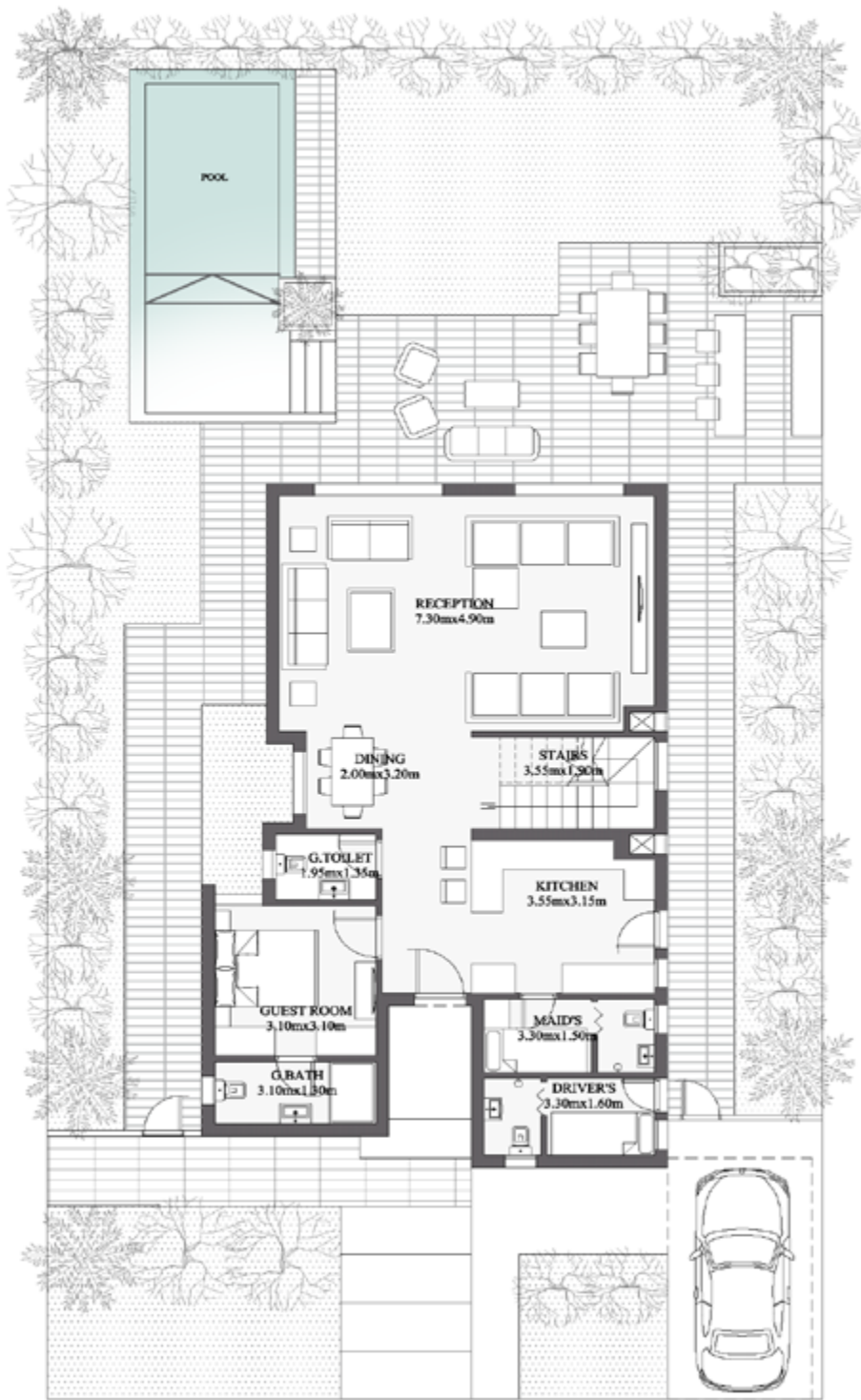
Ground Floor
