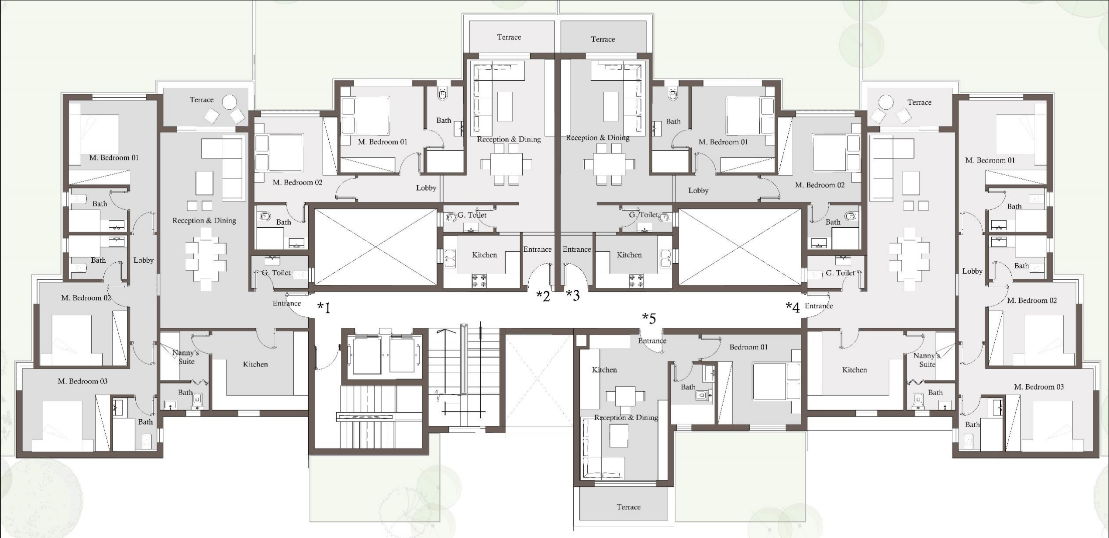
TYPICAL FLOOR
