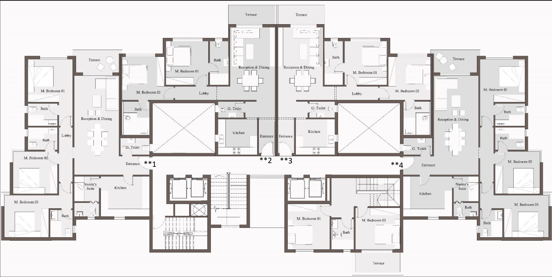
12 TH -14 TH -16 TH FLOOR
