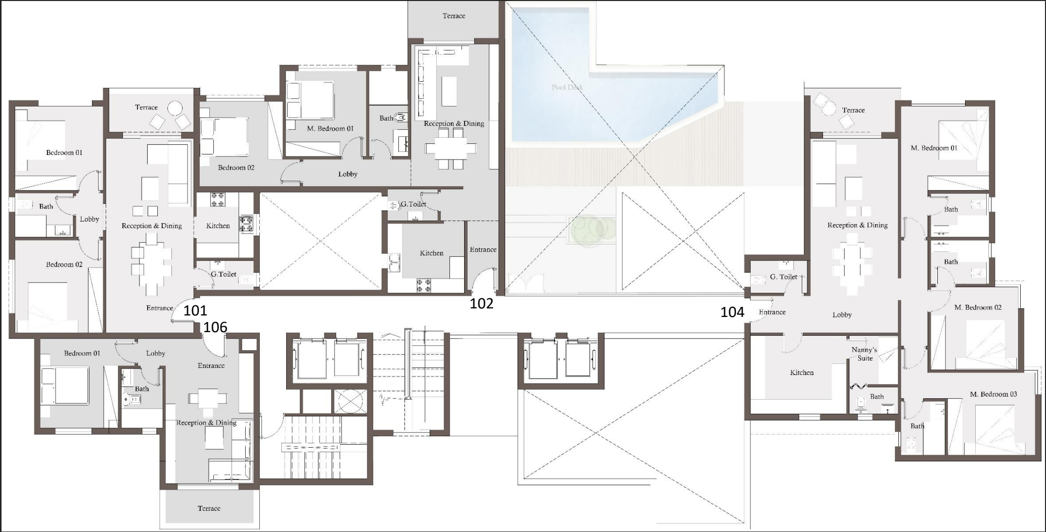
10 TH FLOOR
