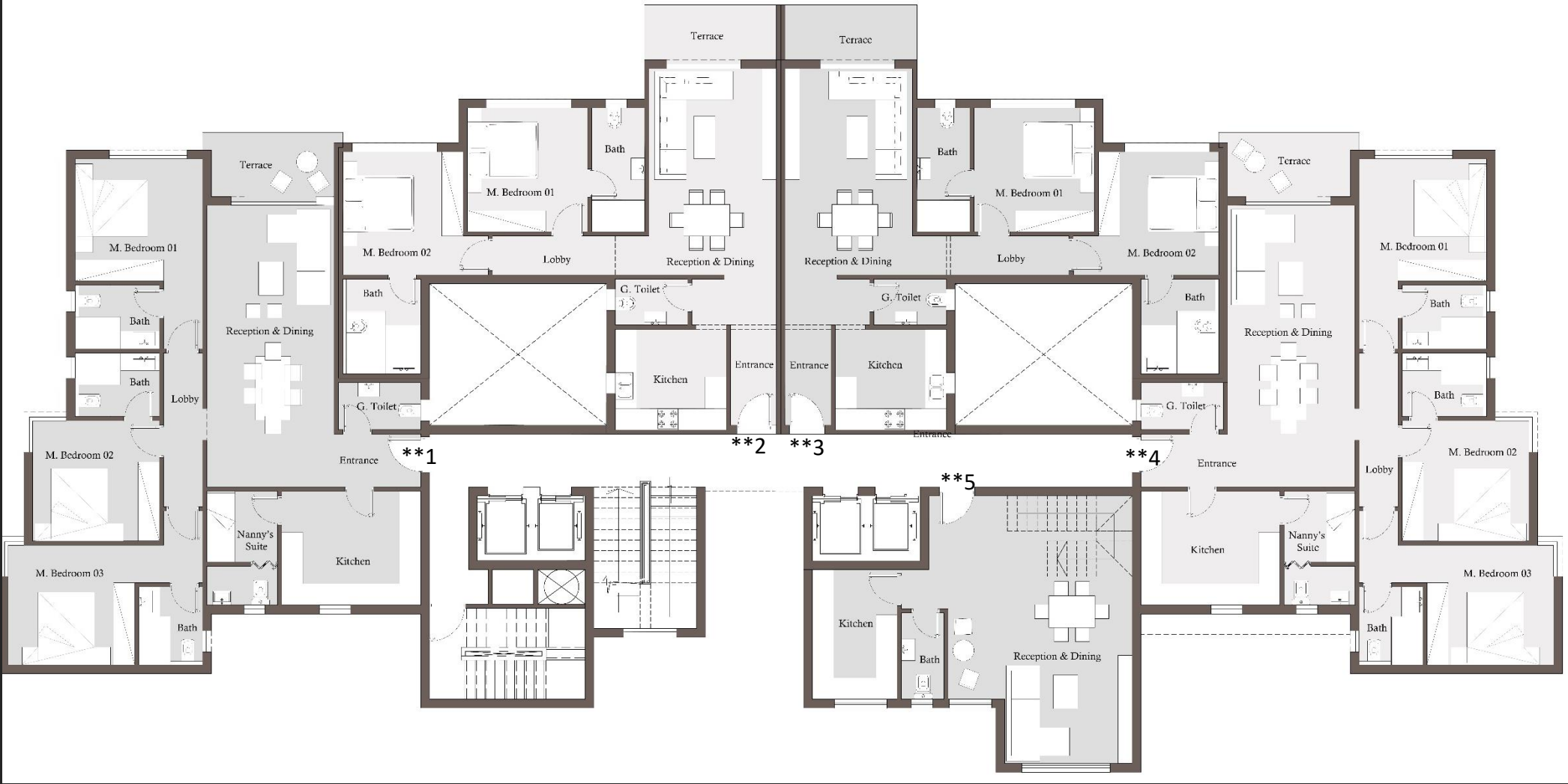
11 TH -13 TH -15 TH FLOOR
