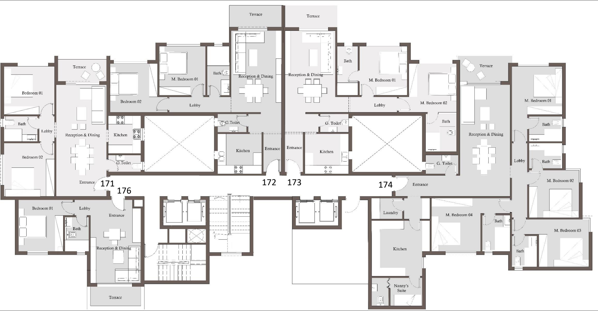
17 TH FLOOR
