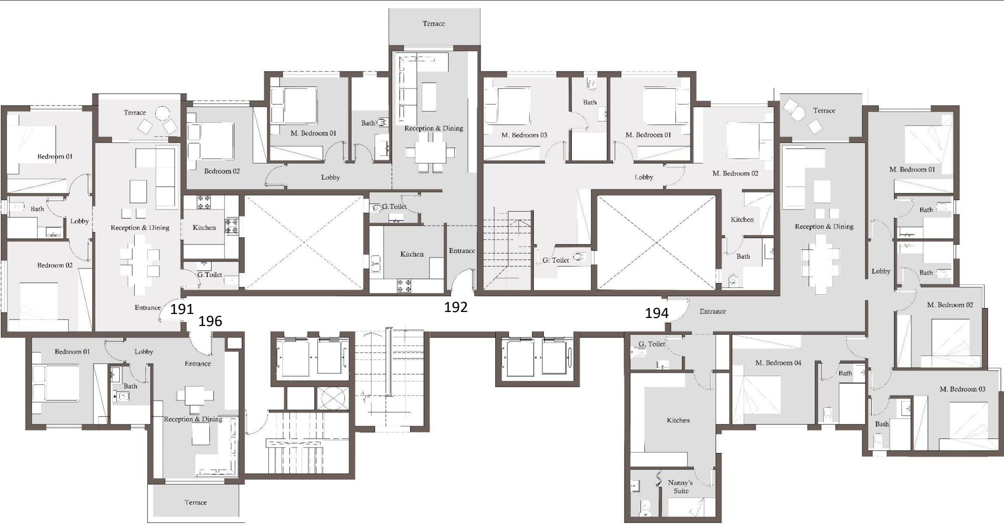
19 TH FLOOR
