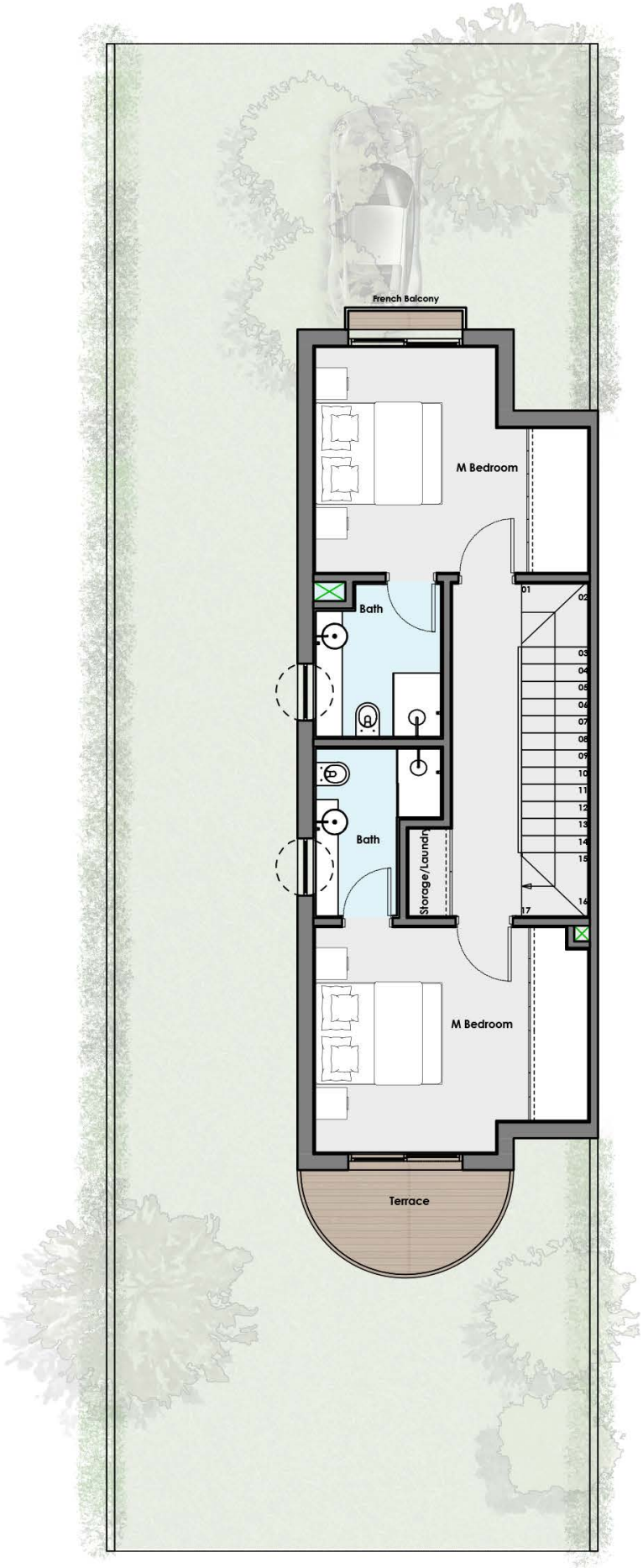
First Floor
