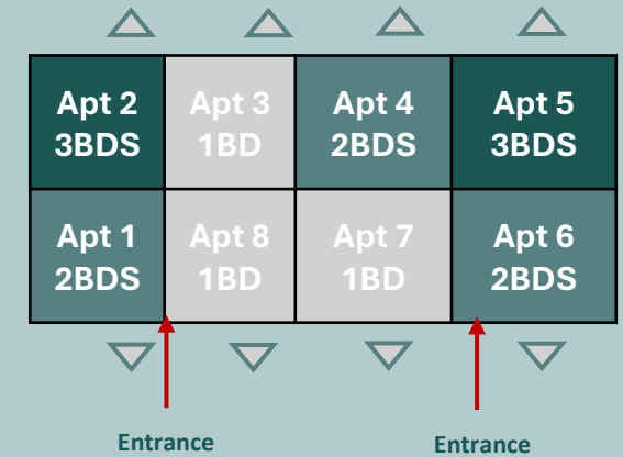
BUILDING C DOUBLE LOADED G+7
