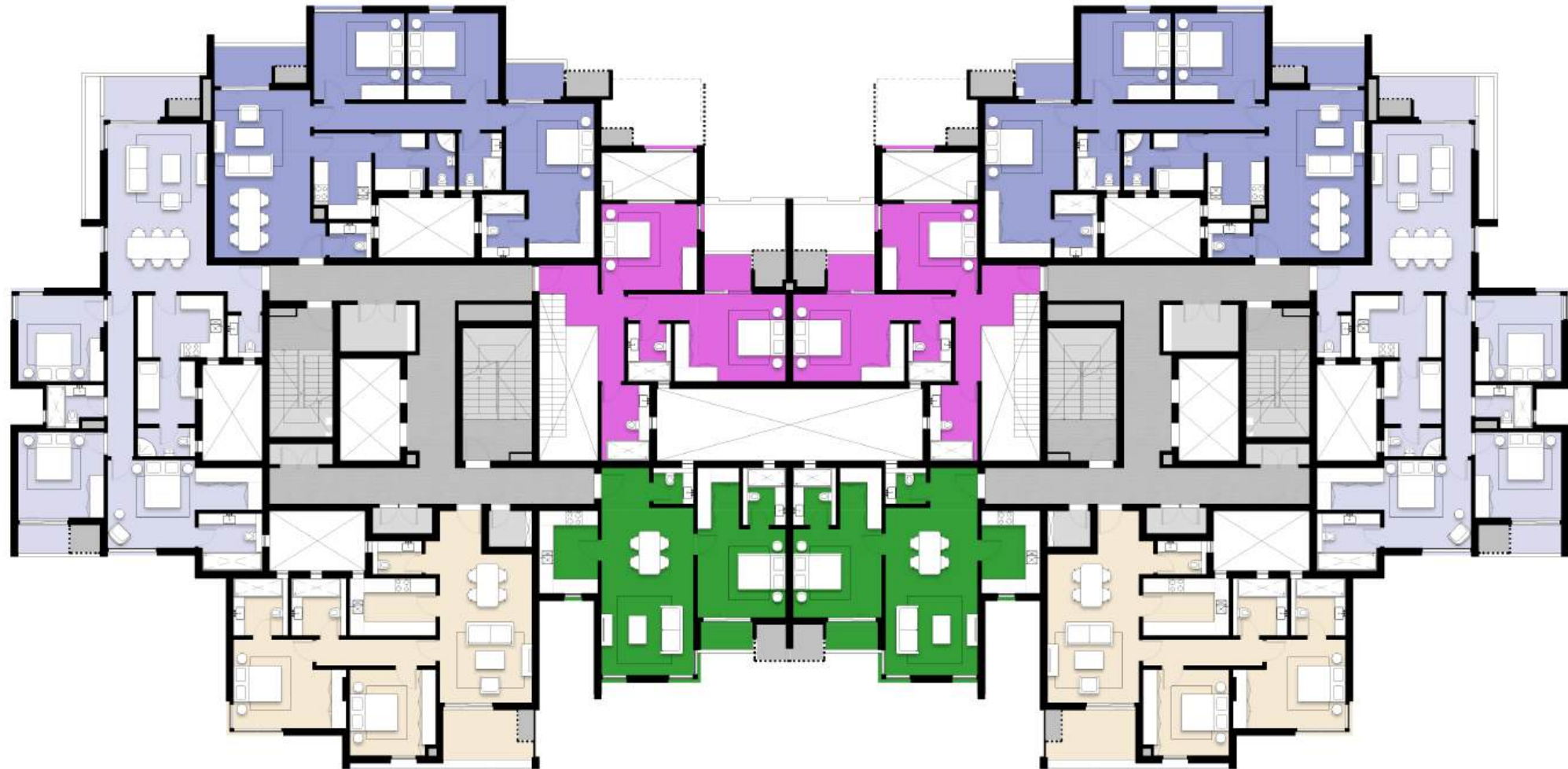
Third Floor
