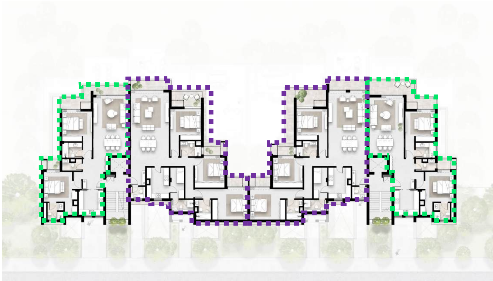
First Floor
