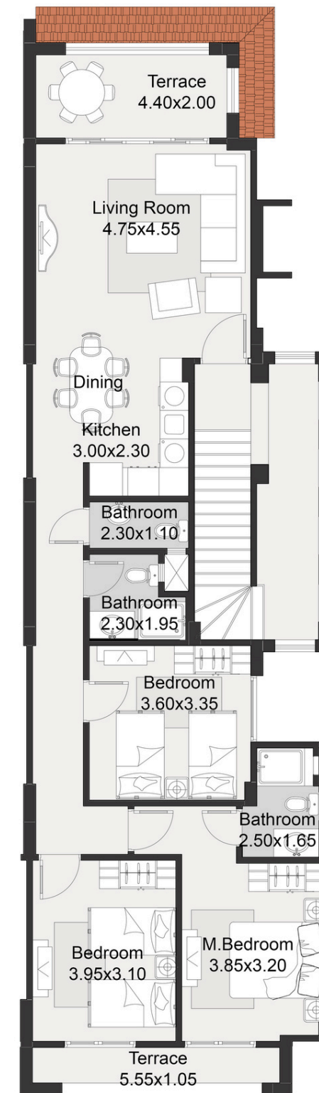
First Floor Plan Area 130 m 2
