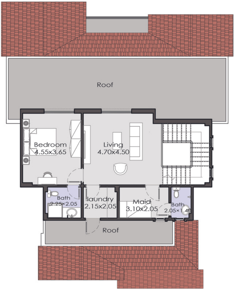
Roof Floor Plan
