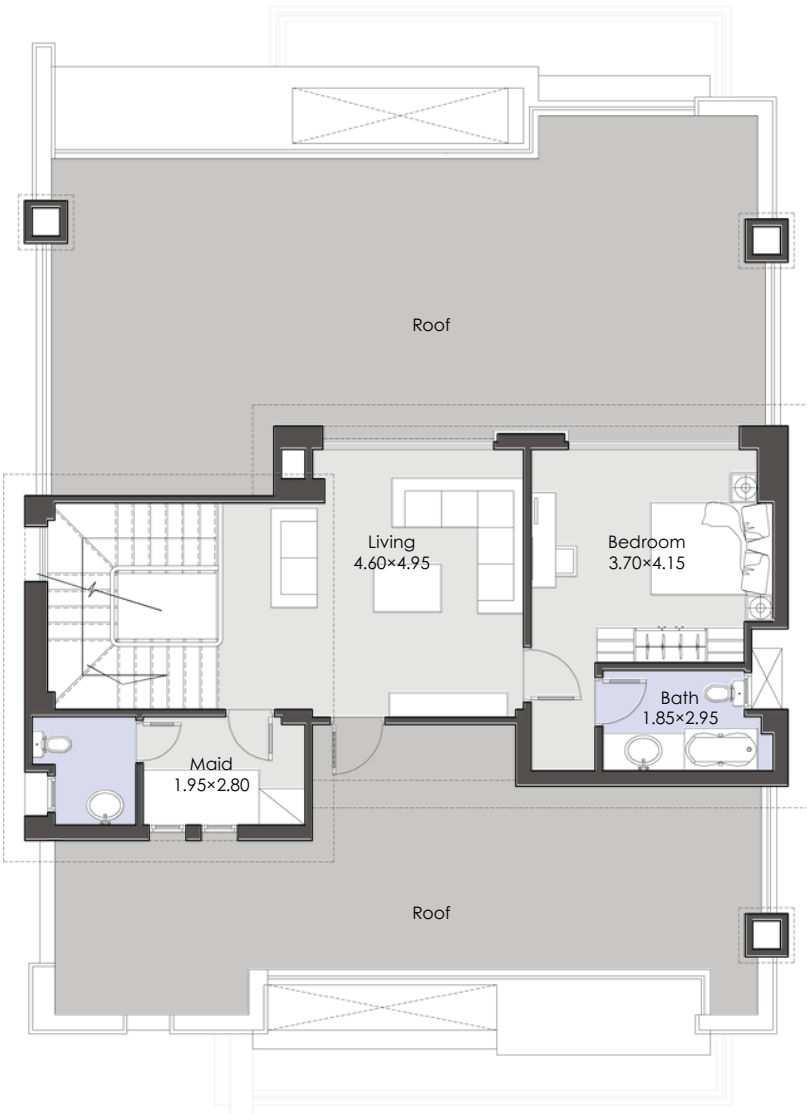
Roof Floor Plan
