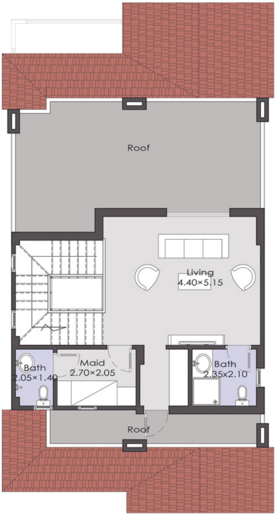
Roof Floor Plan
