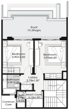
Roof Floor Plan
