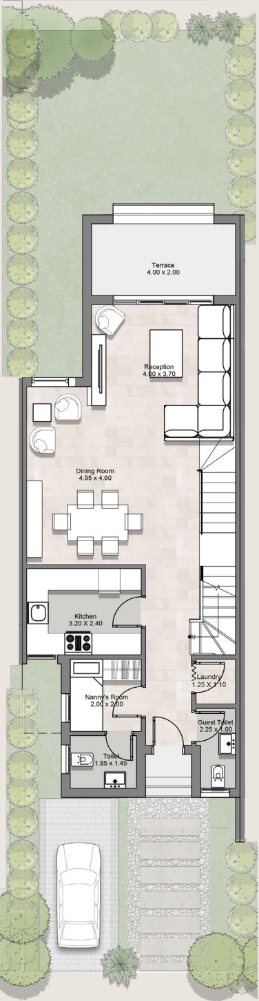
GROUND FLOOR
